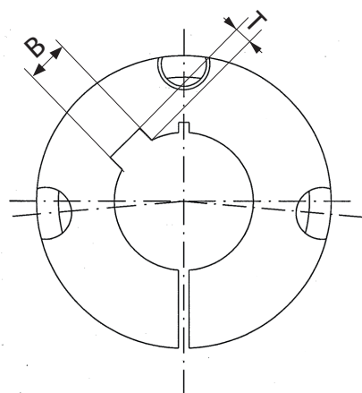
tipo 3 fori type with 3 holes
